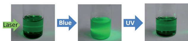
Figure 3. Photographs showing that transparent cis -srMOP-1 in 5% acetone/chloroform (left) becomes a turbid suspension of trans -srMOP-1 (middle) upon irradiation with blue light. UV-light-induced trans -to- cis isomerization gives soluble cis -srMOP-1 again and thus a clear solution (right).
