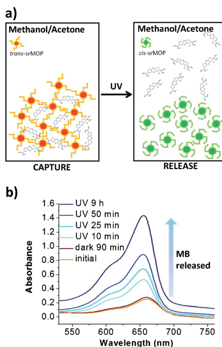
Figure 2. a) Schematic illustration of the capture of MB by trans -srMOP-1 and its release from cis -srMOP-1. The two isomers trans - and cis -srMOP-1 are insoluble. b) UV/Vis spectra of MB in solution in 10% methanol/acetone. As MB was released from cis -srMOP-1, the absorbance of MB in the solution increased.
