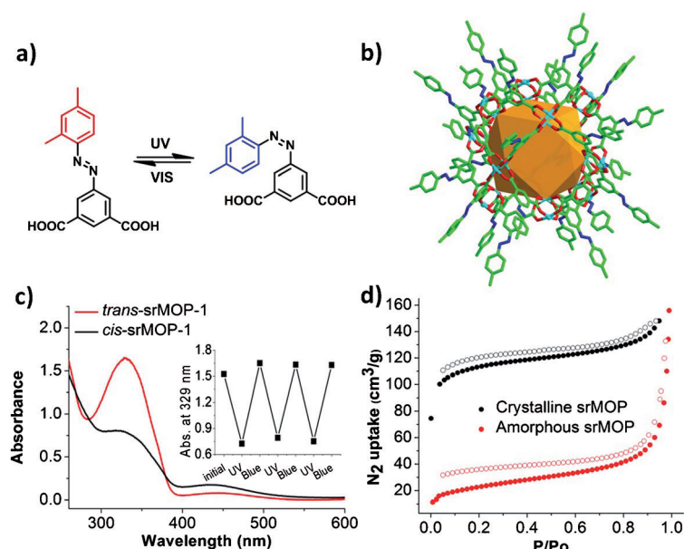
Figure 1. a) Light-induced trans/cis isomerization of 5-(2,4-dimethylphenyldiazenyl)-isophthalic acid, H_2L^1 . b) Crystal structure of srMOP-2 as an azobenzene-function-alyzed cuboctahedral cage, as determined by single-crystal X-ray diffraction analysis. c) Absorption spectra of srMOP-1 with pendent azobenzene groups in chloroform: in the dark after irradiation with blue light (red); after UV irradiation (black). The inset shows the changes in absorbance at 329 nm of srMOP-1 in solution on alternate irradiation with UV and blue light. d) N_2 -adsorption isotherm of crystalline srMOP-1 and amorphous srMOP-1. Crystalline srMOP-1 shows enhanced microporosity.
